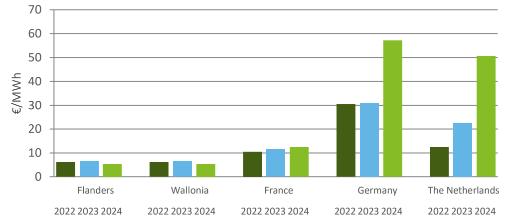
Network costs for Peak load profiles (1000 GWh)
