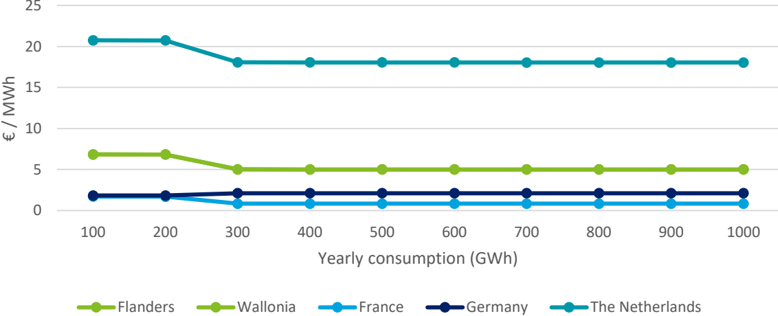
Network costs – 2024 – Baseload profile
