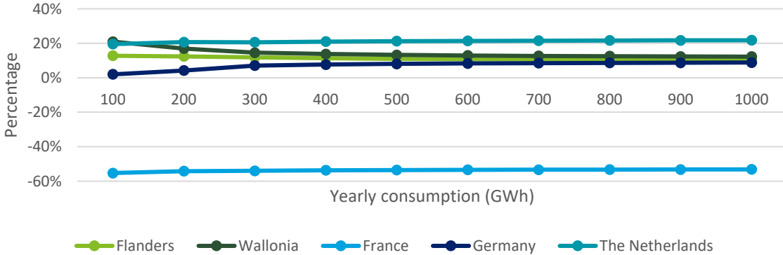
Relative deviation of electricity prices vs average prices in Belgium and its neighboring countries – 2024 – Baseload profile
