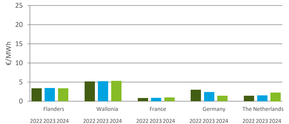
Electricity taxes for Peak load profiles (1000 GWh)
