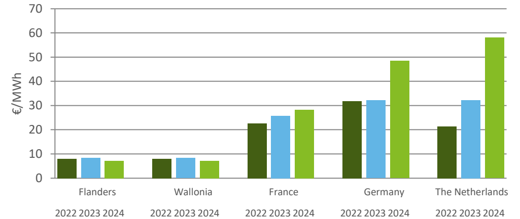
Network costs for Peak load profiles (100 GWh)
