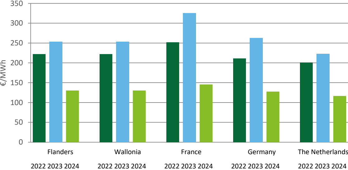
Commodity electricity prices
