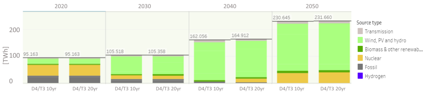
Figure 2: Impact of a lifetime extension of 20 years for D4/T3 on electricity generation.
