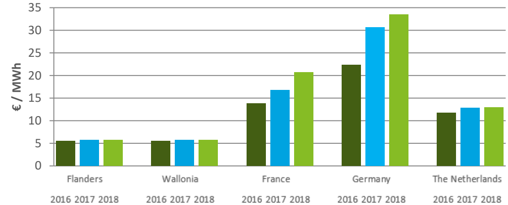
Network costs for peak load profiles (100 GWh)
