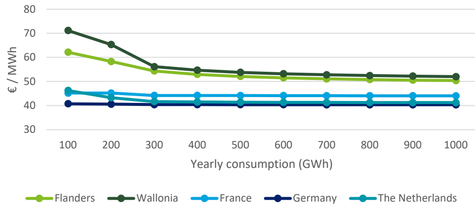
All-in electricity prices – 2018 – Baseload profile
