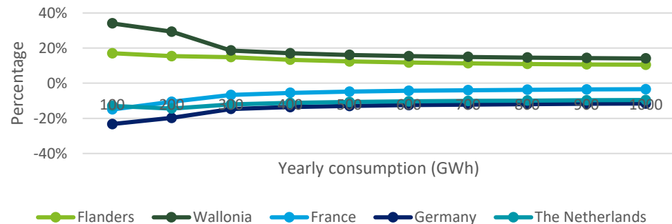
Relative deviation of electricity prices vs average prices in Belgium and its neighboring countries – 2018 – Baseload profile
