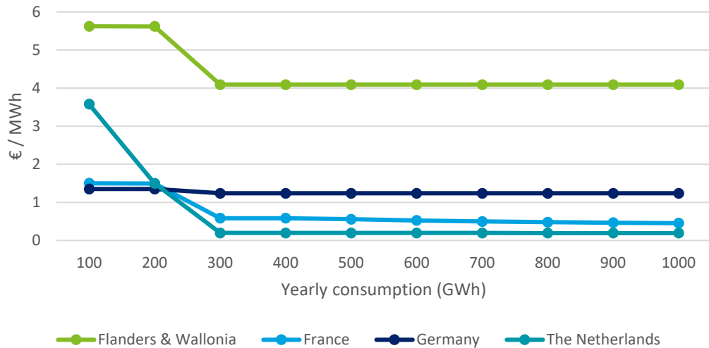
Network costs – 2018 – Baseload profile
