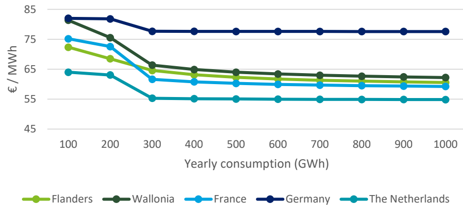
All-in electricity prices – 2018 – Peak load profile
