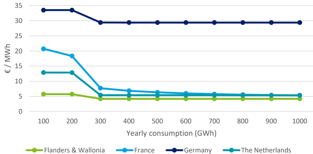
Network costs – 2018 – Peak load profile
